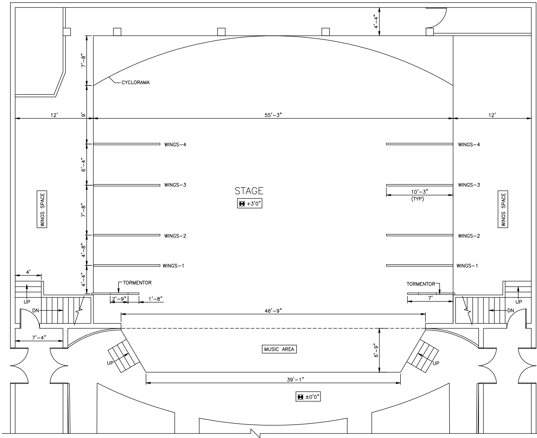
AUDITORIUM - STAGE PLAN
